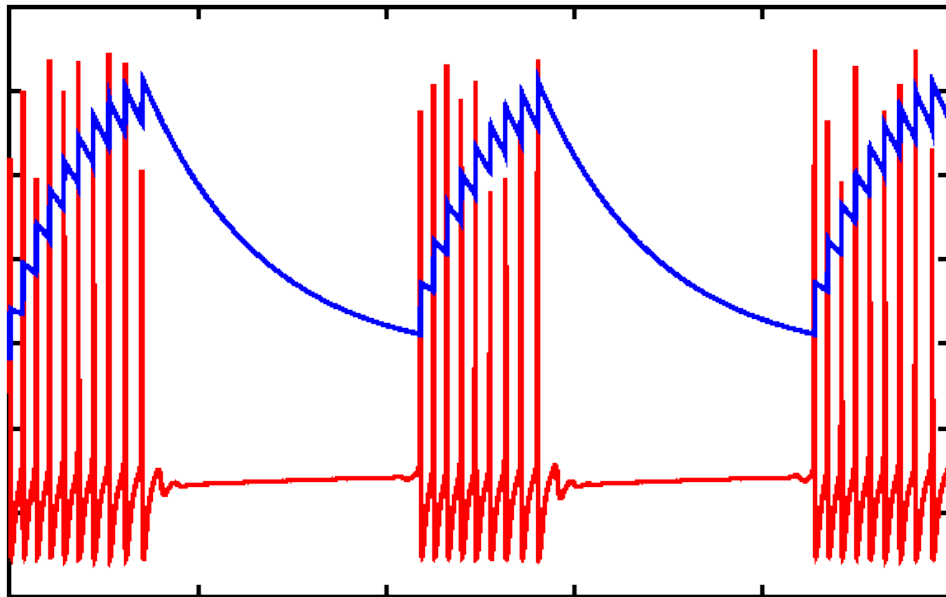
Endogeneous Burster
