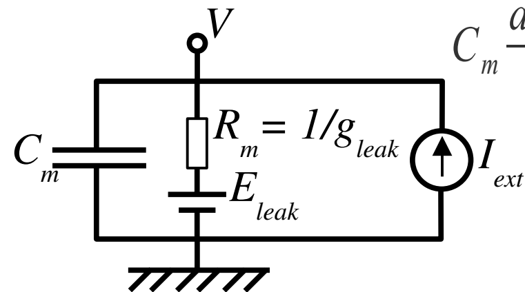
Leaky Integrator
