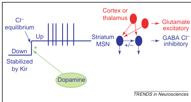
Figure 3. Important factors for the down and up states in medium spiny neurons. To the left is a schematic drawing of the transition from a down to an up state in a medium spiny neuron (MSN) of the GABAergic, substance-P-expressing subtype. The down state is stabilized by K^+ currents of the inward-rectifier type (Kir). An excitatory input from the cortex or thalamus (red, right) can depolarize the MSN so that it is transferred to an up state and Kir will then be turned off. MSNs are unusual in that their Cl^- equilibrium potential is comparatively depolarized and close to the membrane potential of the up state. This could mean that the lateral GABAergic interaction between MSNs can to some degree facilitate the occurrence of an up state. During the up state, an MSN can respond to additional excitation with action potentials; only then can it act on pallidal neurons and possibly disinhibit a motor target. The transition from a down state to an up state is facilitated by dopamine, as indicated. MSN neurons thus have three states: a down state, an up state and, with further depolarization, a state in which they fire action potentials.
